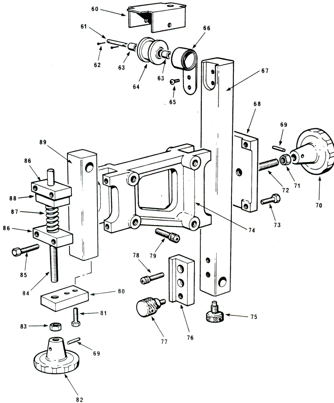
TOP BRACKET
