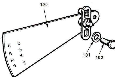
TENSION INDICATOR
